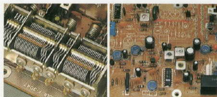
FM Frontend
